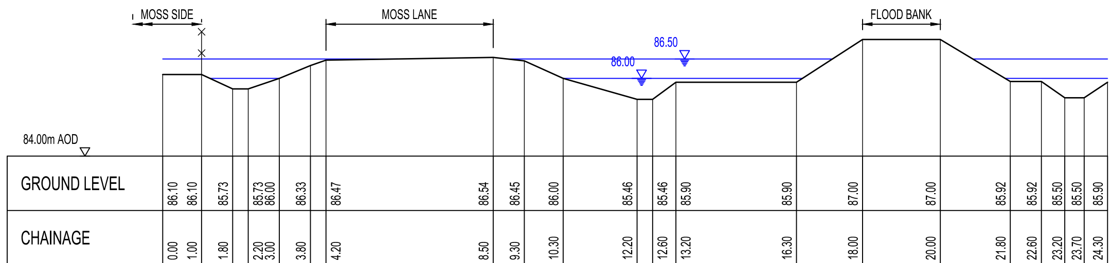
SECTION 1-1 (SCALE 1:100)
