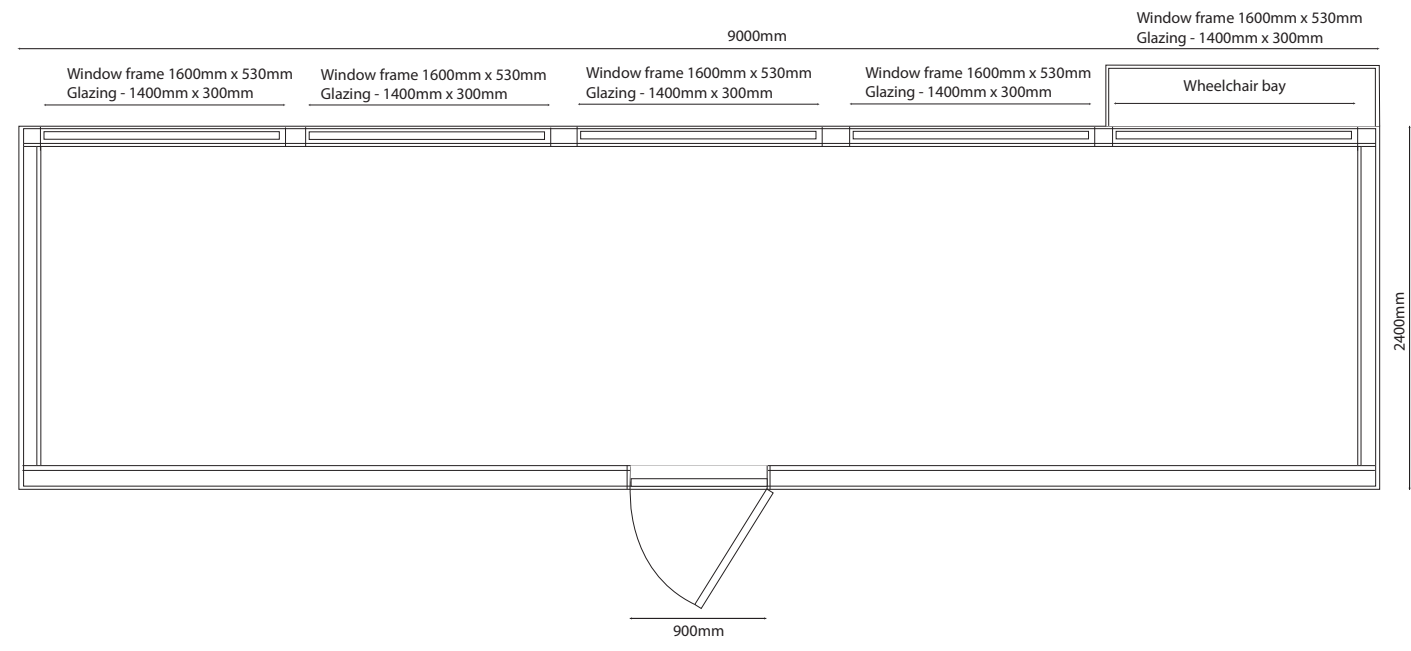
FLOOR PLAN
